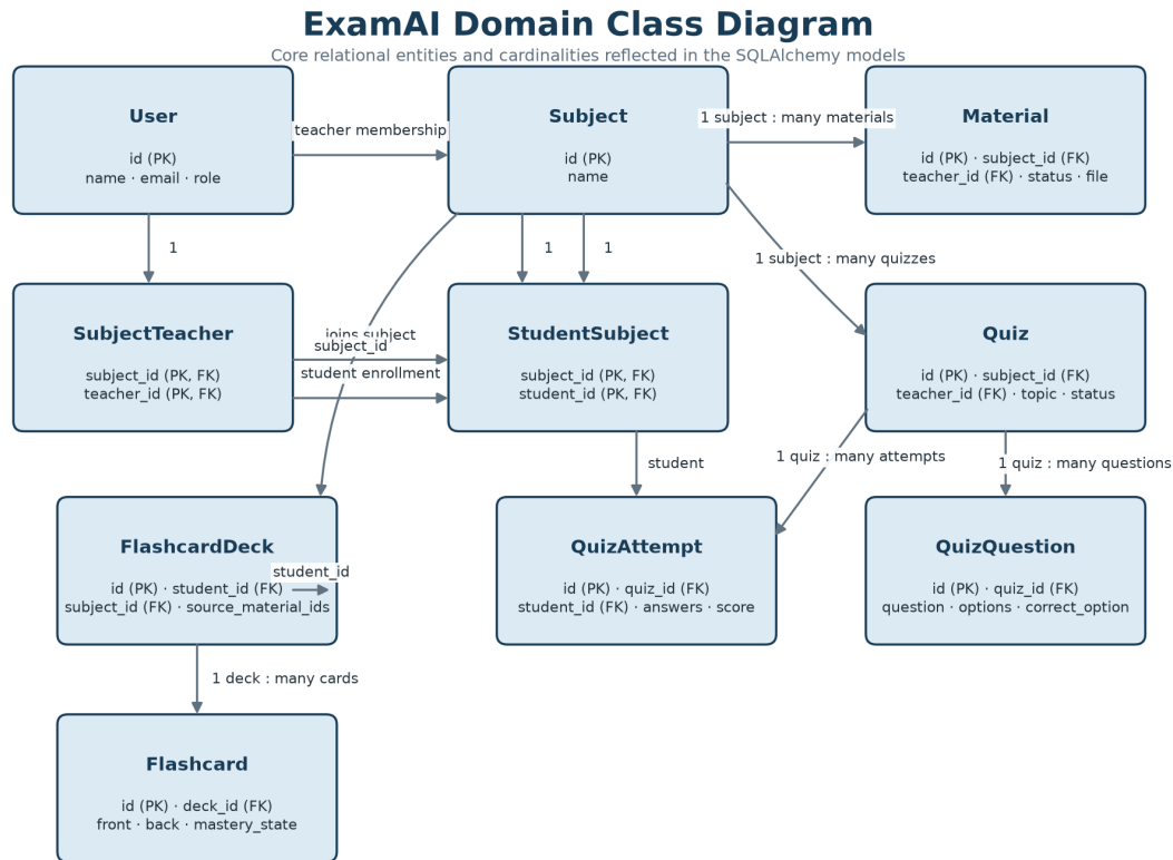
Figure 7.2: Class diagram
